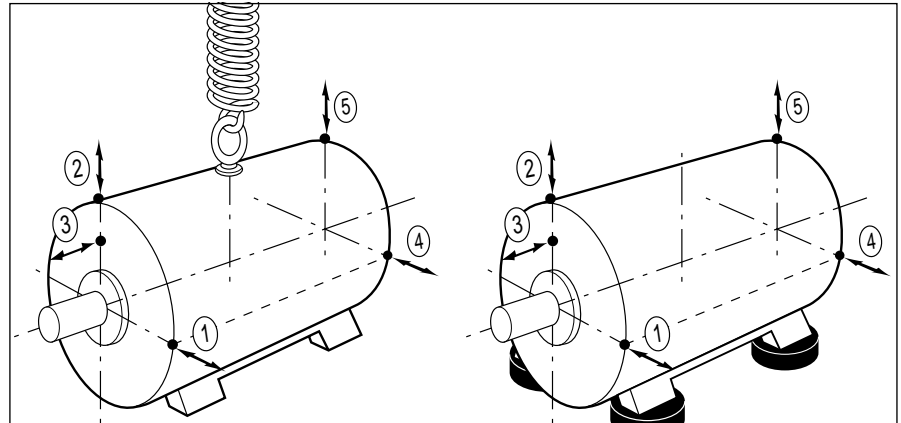
▲ Measuring system for suspended machines
